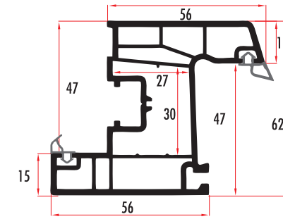
PEG62441 62 MM 4 ODACIKLI PENCERE KANAT / WINDOW SASH PROFILE PEG62442 (RENKLİ/COLORED)
