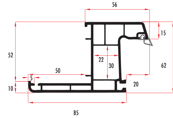
ENR62321 62 MM 3 ODACIKLI PERVAZLI KASA / FRAME PROFILE WITH BORDER ENR62322 (RENKLİ/COLORED)
