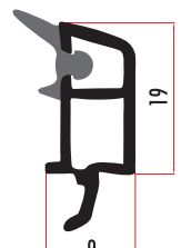
CAM5431 32 MM ÜÇ CAM ÇİTASI 32 MM TRIPLE GLAZING BEAD CAM5432 (RENKLİ/COLORED)
