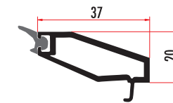
CAM6031 4 MM DÜZ TEK CAM ÇİTASI 4 MM SINGLE GLAZING BEAD CAM6032 (RENKLİ/COLORED)
