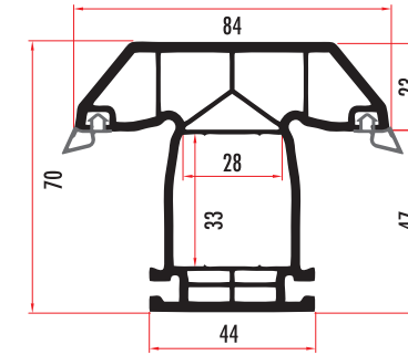
SAF70521 70 MM 5 ODACIKLI ORTA KAYIT / MULLION PROFILE SAF70522 (RENKLİ/COLORED)
