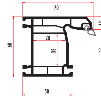
ATL60411 60 MM 4 ODACIKLI SUPER KASA SUPER FRAME PROFILE ATL60412 (RENKLİ/COLORED)
