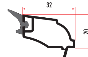
CAM5411 10 MM DEKORATİF TEK CAM ÇİTASI 10 MM DECORATIVE GLAZING BEAD CAM5412 (RENKLİ/COLORED)
