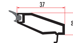
CAM6031 4 MM DÜZ TEK CAM ÇİTASI 4 MM SINGLE GLAZING BEAD CAM6032 (RENKLİ/COLORED)
