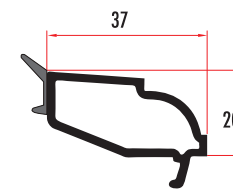
CAM6011 4 MM DEKORATİF TEK CAM ÇİTASI 4 MM DECORATIVE SINGLE GLAZING BEAD CAM6012 (RENKLİ/COLORED)
