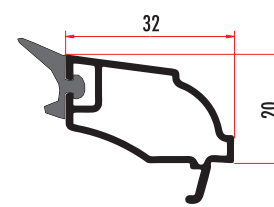
CAM5411 10 MM DEKORATİF TEK CAM ÇİTASI 10 MM DECORATIVE GLAZING BEAD CAM5412 (RENKLİ/COLORED)
