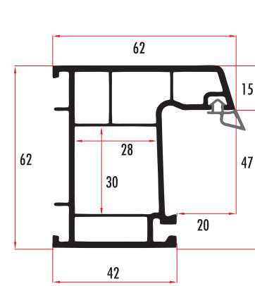
ENR62311 62 MM 3 ODACIKLI KASA / FRAME PROFILE ENR62312 (RENKLİ/COLORED)
