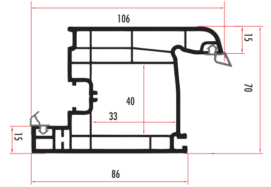
YAK71551 70 mm KAPI KANAT DOOR SASH PROFILE YAK71552 (RENKLİ/COLORED)
