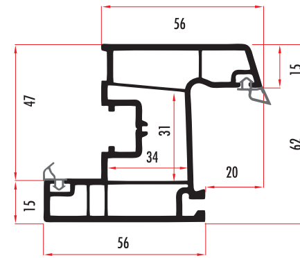
ENR60341 662 MM 3 ODACIKLI PENCERE KANAT / WINDOW SASH PROFILE ENR60342 (RENKLİ/COLORED)
