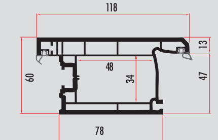
TRU60361 60 MM 3 ODACIKLI DIŞA AÇILIR KAPI KANAT OUTWARD OPENING DOOR SASH PROFILE TRU60362 (RENKLİ/COLORED)
