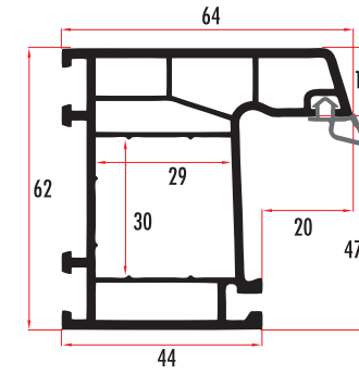
PEG62411 62 MM 4 ODACIKLI KASA / FRAME PROFILE PEG62412 (RENKLİ/COLORED)
