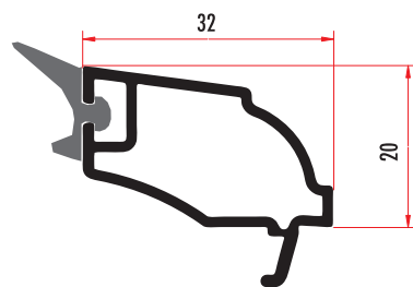
CAM5411 10 MM DEKORATİF TEK CAM ÇİTASI 10 MM DECORATIVE GLAZING BEAD CAM5412 (RENKLİ/COLORED)
