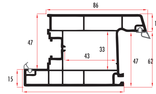
PEG62451 62 MM 3 ODACIKLI KAPI KANAT / DOOR SASH PROFILE PEG62452 (RENKLİ/COLORED)
