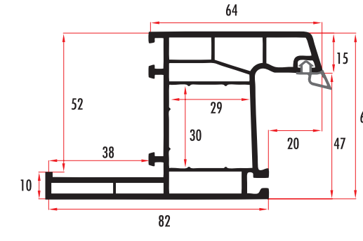
PEG62421 62 MM 4 ODACIKLI PERVAZLI KASA / FRAME PROFILE WITH BORDER PEG62422 (RENKLİ/COLORED)
