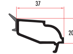
CAM6011 4 MM DEKORATİF TEK CAM ÇİTASI 4 MM DECORATIVE SINGLE GLAZING BEAD CAM6012 (RENKLİ/COLORED)
