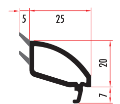
CAM7131 24 MM OVAL SERİ ÇİFT CAM ÇİTASI 24 MM DOUBLE GLAZING BEAD CAM7132 (RENKLİ/COLORED)
