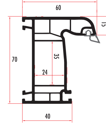
LAP71511 70 MM KASA FRAME PROFILE LAP71512 (RENKLİ/COLORED)
