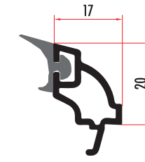
CAM5421 24 MM DEKORATİF ÇİFT CAM ÇİTASI 24 MM DECORATIVE GLAZING BEAD CAM5422 (RENKLİ/COLORED)
