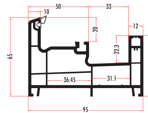
SİT7681 76 MM TEK RAYLI SÜRME KASA SINGLE RAILED SLIDING FRAME PROFILE SİT7682 (RENKLİ/COLORED)
