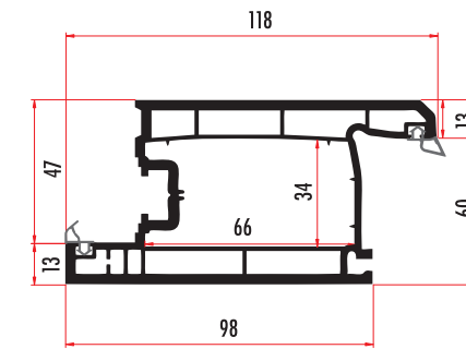
TRU60351 60 MM. 3 ODACIKLI KAPI KANAT / DOOR SASH PROFILE TRU60352 (RENKLİ/COLORED)
