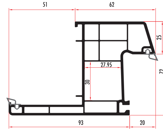
KUV 72431 72 MM 4 ODACIKLI PERVAZLI KASA / FRAME PROFILE KUV 72432 (RENKLİ/COLORED)
