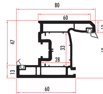
TRU60341 60 MM. 3 ODACIKLI PENCERE KANAT / WINDOW SASH PROFILE TRU60342 (RENKLİ/COLORED)
