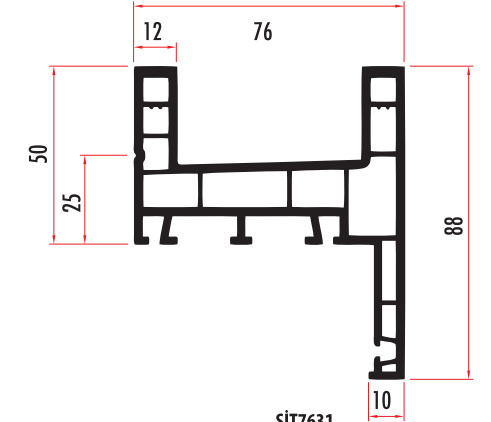
SİT7631 76 MM ÇİFT RAYLI PERVAZLI SÜRME KASA DOUBLE RAILED SLIDING FRAME PROFILE WITH BORDER SİT7632 (RENKLİ/COLORED)
