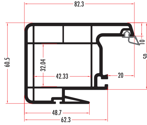
SİT7691 SÜRME DİKEY KİLİTLİ ORTA KAYIT SLIDING VERTICAL LOCKED MULLION PROFILE SİT7662 (RENKLİ/COLORED)
