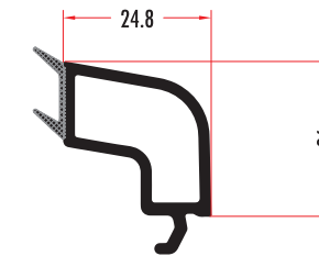
QUA8211 36 MM ÇİFT CAM ÇİTASI 36 MM DOUBLE GLAZING BEAD QUA8212 (RENKLİ/COLORED)
