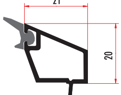
CAM6041 20 MM DÜZ ÇİFT CAM ÇİTASI 20 MM DOUBLE GLAZING BEAD CAM6042 (RENKLİ/COLORED)
