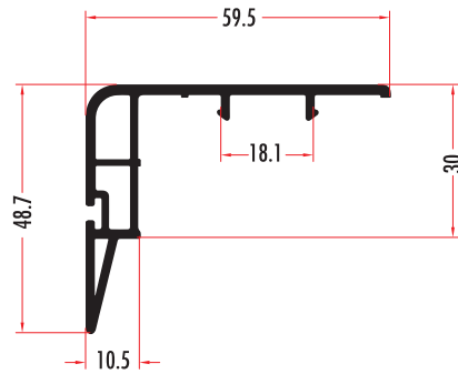
SİT7661 SÜRME KANAT KİLİT ADAPTÖRÜ LOCK ADAPTER FOR SLIDING SASH PROFILE SİT7662 (RENKLİ/COLORED)
