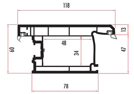
TRU60361 60 MM. 3 ODACIKLI DIŞA AÇILIM PROFİLİ / OUTWARD OPENING DOOR SASH PROFILE TRU60362 (RENKLİ/COLORED)
