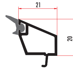
CAM6041 20 MM DÜZ ÇİFT CAM ÇİTASI 20 MM DOUBLE GLAZING BEAD CAM6042 (RENKLİ/COLORED)
