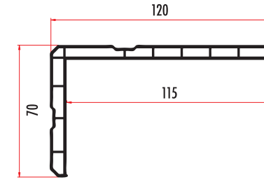
YARP31 70 X 120 PERVAZ PROFİLİ 70 X 120 BORDER PROFILE YARP32 (RENKLİ/COLORED)
