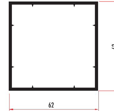
YARK62621 62X62 KUTU PROFİLİ 62 X 62 BOX PROFILE YARK62622 (RENKLİ/COLORED)
