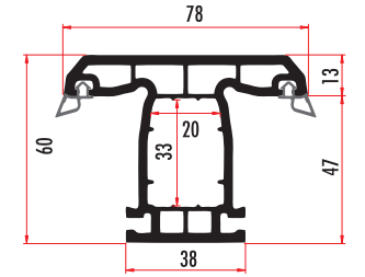
TRU60331 60 MM. 3 ODACIKLI ORTA KAYIT / MULLION PROFILE TRU60332 (RENKLİ/COLORED)
