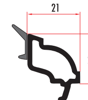
CAM6021 20 MM DEKORATİF ÇİFT CAM ÇİTASI 20 MM DECORATIVE DOUBLE GLAZING BEAD CAM6022 (RENKLİ/COLORED)
