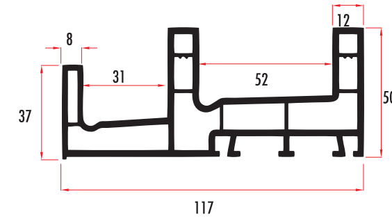
SİT7621 SİNEKLİKLİ SÜRME KASA DOUBLE RAILED SLIDING FRAME PROFILE WITH FLY SCREEN SİT7622 (RENKLİ/COLORED)
