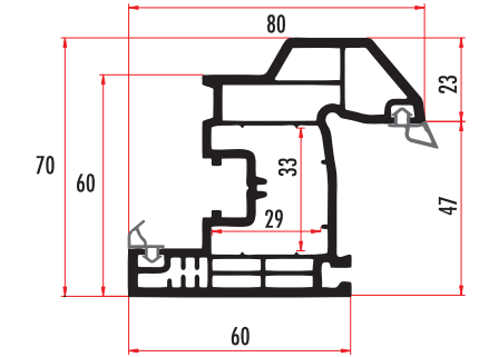
SAF70531 70 MM DAMLALIKLI PENCERE KANAT / DRIP WINDOW SASH PROFILE SAF70532 (RENKLİ/COLORED)
