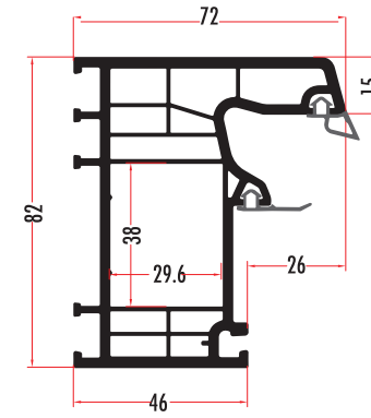
QUA8211 82 MM 6 ODACIKLI L KASA FRAME PROFILE QUA8212 (RENKLİ/COLORED)
