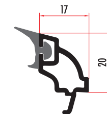
CAM5421 24 MM DEKORATİF ÇİFT CAM ÇİTASI 24 MM DECORATIVE GLAZING BEAD CAM5422 (RENKLİ/COLORED)
