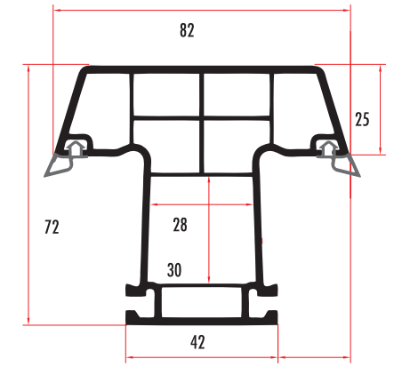
KUV 72421 72 MM 3 ODACIKLI ORTA KAYIT / MULLION PROFILE KUV 72422 (RENKLİ/COLORED)
