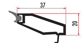
CAM6031 4 MM DÜZ TEK CAM ÇİTASI 4 MM SINGLE GLAZING BEAD CAM6032 (RENKLİ/COLORED)
