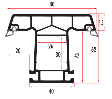
PEG62431 62 MM 4 ODACIKLI ORTA KAYIT / MULLION PROFILE PEG62432 (RENKLİ/COLORED)
