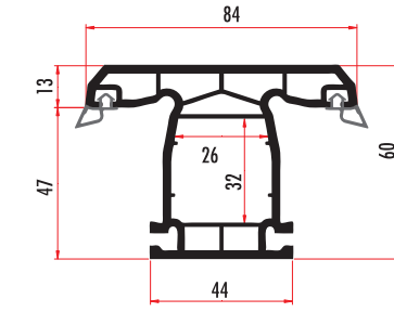
ATL60421 60 MM 4 ODACIKLI SUPER ORTA KAYIT SUPER MULLION PROFILE ATL60422 (RENKLİ/COLORED)
