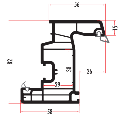
QUA8241 82 MM 6 ODACIKLI PENCERE KANAT WINDOW SASH PROFILE QUA8242 (RENKLİ/COLORED)
