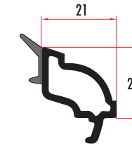
CAM6021 20 MM DEKORATİF ÇİFT CAM ÇİTASI 20 MM DECORATIVE DOUBLE GLAZING BEAD CAM6022 (RENKLİ/COLORED)
