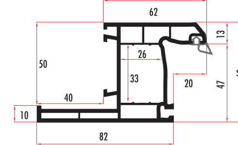
TRU60321 60 MM. 3 ODACIKLI PERVAZLI KASA / FRAME PROFILE WITH BORDER TRU60322 (RENKLİ/COLORED)
