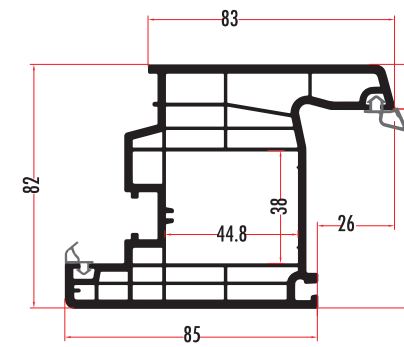
QUA8251 82 MM 6 ODACIKLI KAPI KANAT DOOR SASH PROFILE QUA8252 (RENKLİ/COLORED)
