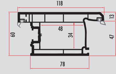
TRU60361 60 MM. 3 ODACIKLI DIŞA AÇILIM PROFİLİ / OUTWARD OPENING DOOR SASH PROFILE TRU60362 (RENKLİ/COLORED)
