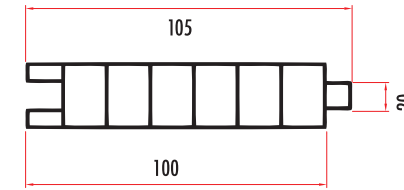
YARP11 PANEL PROFİL PANEL PROFILE YARP12 (RENKLİ/COLORED)
