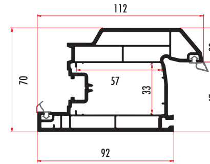
SAF70541 70 MM DAMLALIKLI KAPI KANAT DRIP DOOR SASH PROFILE SAF70542 (RENKLİ/COLORED)
