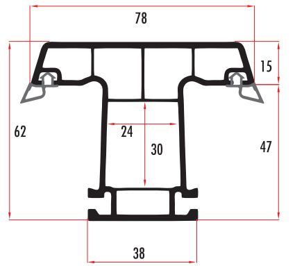
ENR62331 62 MM 3 ODACIKLI ORTA KAYIT / MULLION PROFILE ENR62332 (RENKLİ/COLORED)
