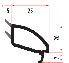
CAM7131 24 mm OVAL SERİ ÇİFT CAM ÇİTASI 24 mm DOUBLE GLAZING BEAD CAM7132 (RENKLİ/COLORED)
