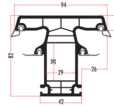
QUA8231 82 MM 6 ODACIKLI ORTA KAYIT MULLION PROFILE QUA8232 (RENKLİ/COLORED)
