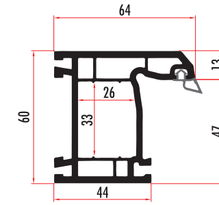
TRU60311 60 MM. 3 ODACIKLI KASA / FRAME PROFILE TRU60312 (RENKLİ/COLORED)
