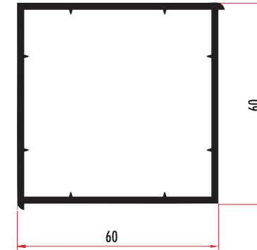
YARK60601 60 X 60 KUTU PROFİLİ 60 X 60 BOX PROFILE YARK60602 (RENKLİ/COLORED)
