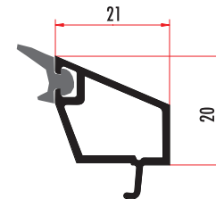
CAM6041 20 MM DÜZ ÇİFT CAM ÇİTASI 20 MM DOUBLE GLAZING BEAD CAM6042 (RENKLİ/COLORED)
