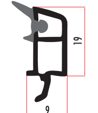
CAM5431 32 MM ÜÇ CAM ÇİTASI 32 MM TRIPLE GLAZING BEAD CAM5432 (RENKLİ/COLORED)
