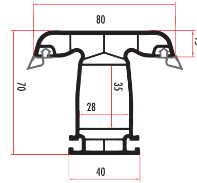
LAP71531 70 MM ORTA KAYIT MULLION PROFILE LAP71532 (RENKLİ/COLORED)
