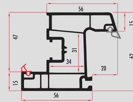
ENR62341 62 MM - 3 ODACIKLI PENCERE KANAT / WINDOW SASH PROFILE PEG62342 (RENKLİ/COLORED)
