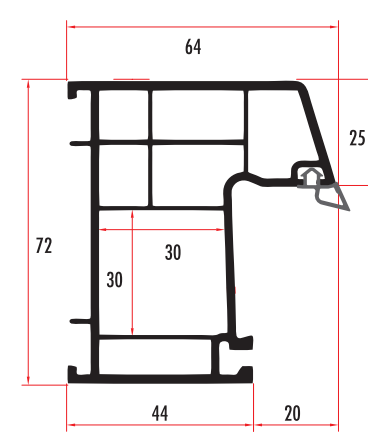
KUV 72411 72 MM 3 ODACIKLI KASA / FRAME PROFILE KUV 72412 (RENKLİ/COLORED)
