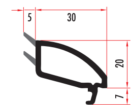
CAM7121 20 mm OVAL SERİ ÇİFT CAM ÇİTASI 20 mm DOUBLE GLAZING BEAD CAM7122 (RENKLİ/COLORED)
