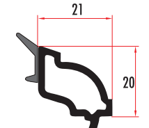
CAM6021 20 MM DEKORATİF ÇİFT CAM ÇİTASI 20 MM DECORATIVE DOUBLE GLAZING BEAD CAM6022 (RENKLİ/COLORED)
