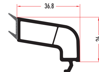
QUA8221 24 MM ÇİFT CAM ÇİTASI 24 MM DOUBLE GLAZING BEAD QUA8222 (RENKLİ/COLORED)
