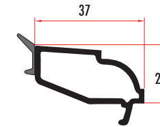
CAM6011 4 MM DEKORATİF TEK CAM ÇİTASI 4 MM DECORATIVE SINGLE GLAZING BEAD CAM6012 (RENKLİ/COLORED)
