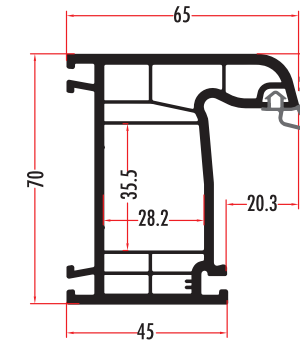
LAP72511 70 MM KASA FRAME PROFILE LAP72512 (RENKLİ/COLORED)
