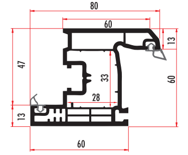
ATL60431 60 MM 4 ODACIKLI PENCERE KANAT WINDOW SASH PROFILE ATL60432 (RENKLİ/COLORED)
