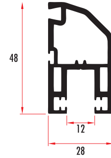
SİT7651 SİNEKLİK PROFİLİ SLIDING FLY SCREEN SASH PROFILE SİT7652 (RENKLİ/COLORED)
