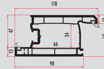
TRU60351 60 MM. 3 ODACIKLI KAPI KANAT / DOOR SASH PROFILE TRU60352 (RENKLİ/COLORED)
