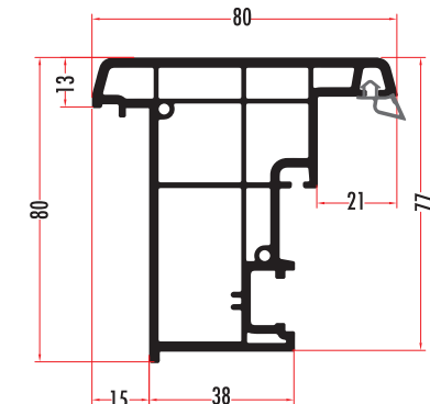
QUA8281 82 MM HAREKETLİ ORTA KAYIT MOVABLE MULLION PROFILE QUA8282 (RENKLİ/COLORED)
