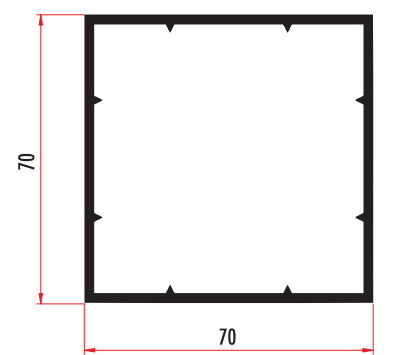
YARK70701 70 X 70 KUTU PROFİLİ 70 X 70 BOX PROFILE YARK70702 (RENKLİ/COLORED)
