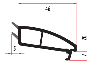
4 MM OVAL SERİ TEK CAM ÇİTASI 4 MM SINGLE GLAZING BEAD CAM7112 (RENKLİ/COLORED)
