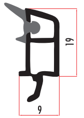
CAM5431 32 MM ÜÇ CAM ÇİTASI 32 MM TRIPLE GLAZING BEAD CAM5432 (RENKLİ/COLORED)
