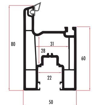
SİT7641 SÜRME KANAT /SLIDING SASH PROFILE SİT7642 (RENKLİ/COLORED)
