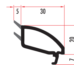
CAM7121 20 MM OVAL SERİ ÇİFT CAM ÇİTASI 20 MM DOUBLE GLAZING BEAD CAM7122 (RENKLİ/COLORED)
