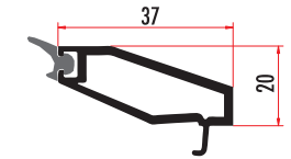
CAM6031 4 MM DÜZ TEK CAM ÇİTASI 4 MM SINGLE GLAZING BEAD CAM6032 (RENKLİ/COLORED)
