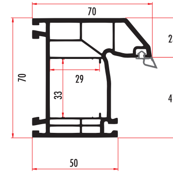
SAF70511 70 MM 5 ODACIKLI KASA / FRAME PROFILE SAF70512 (RENKLİ/COLORED)
