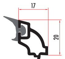
CAM5421 24 MM DEKORATİF ÇİFT CAM ÇİTASI 24 MM DECORATIVE GLAZING BEAD CAM5422 (RENKLİ/COLORED)
