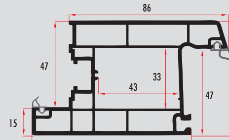
ENR62341 62 MM - 3 ODACIKLI PENCERE KANAT / WINDOW SASH PROFILE PEG62342 (RENKLİ/COLORED)
