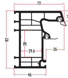
QUA8211 82 MM 6 ODACIKLI L KASA FRAME PROFILE QUA8212 (RENKLI/COLORED)
