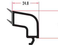
QUA8211 36 MM ÇİFT CAM ÇİTASI 36 MM DOUBLE GLAZING BEAD QUA8212 (RENKLI/COLORED)
