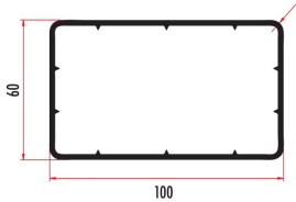
YARK601001 60 X 100 KUTU PROFİLİ 60 X 100 BOX PROFILE YARK601002 (RENKLİ/COLORED)
