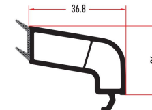
QUA8221 24 MM ÇİFT CAM ÇİTASI 24 MM DOUBLE GLAZING BEAD QUA8222 (RENKLI/COLORED)
