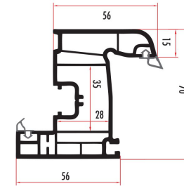
LAP71541 70 MM PENCERE KANAT WINDOW SASH PROFILE LAP71542 (RENKLİ/COLORED)
