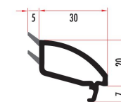
CAM7121 20 MM OVAL SERİ ÇİFT CAM ÇİTASI 20 MM DOUBLE GLAZING BEAD CAM7122 (RENKLİ/COLORED)
