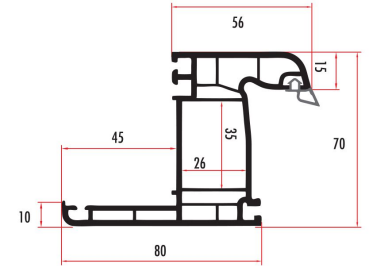
LAP71521 70 MM PERVAZLI KASA FRAME PROFILE WITH BORDER LAP71522 (RENKLİ/COLORED)
