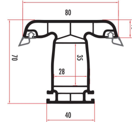
LAP71531 70 MM ORTA KAYIT MULLION PROFILE LAP71532 (RENKLİ/COLORED)
