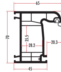
LAP72511 70 MM KASA FRAME PROFILE LAP72512 (RENKLİ/COLORED)
