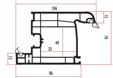
LAP71551 70 MM KAPI KANAT DOOR SASH PROFILE LAP71552 (RENKLİ/COLORED)
