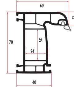
LAP71511 70 MM KASA FRAME PROFILE LAP71512 (RENKLİ/COLORED)
