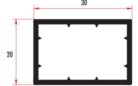
ZİR8661 TEK RAYLI SÜRME KASA YAN KAPATMA PROFİLİ ADAPTER FOR SINGLE RAILED SLIDING FRAME PROFILE ZİR8662 (RENKLİ/COLORED)
