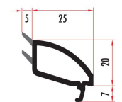
CAM7131 24 MM OVAL SERİ ÇİFT CAM ÇİTASI 24 MM DOUBLE GLAZING BEAD CAM7132 (RENKLİ/COLORED)
