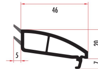
CAM7112 4 MM OVAL SERİ TEK CAM ÇİTASI 4 MM SINGLE GLAZING BEAD CAM7112 (RENKLİ/COLORED)
