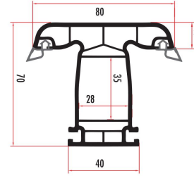
YAK71531 70 mm ORTA KAVİT MULLION PROFILE YAK71532 (RENKLİ/COLORED)
