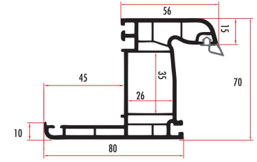
YAK71521 70 MM PERVAZLI KASA FRAME PROFILE WITH BORDER YAK71522 (RENKLİ/COLORED)
