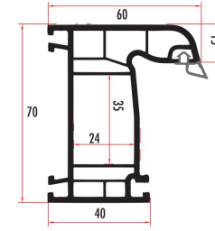
YAK71511 70 MM KASA / FRAME PROFILE YAK71512 (RENKLİ/COLORED)
