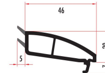
CAM7121 4 mm OVAL SERİ TEK CAM ÇİTASI 4 mm SINGLE GLAZING BEAD CAM7112 (RENKLİ/COLORED)
