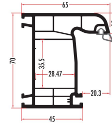
YAK72511 70 MM KASA / FRAME PROFILE YAK72512 (RENKLİ/COLORED)
