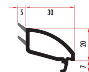
CAM7122 20 mm OVAL SERİ ÇİFT CAM ÇİTASI 20 mm DOUBLE GLAZING BEAD CAM7122 (RENKLİ/COLORED)
