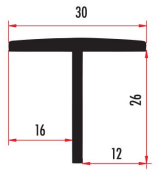
YARTK1 DAR T KAPATMA PROFİLİ T CLOSER PROFILE YARTK2 (RENKLİ/COLORED)
