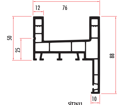
SİT7631 76 MM ÇİFT RAYLI PERVAZLI SÜRME KASA DOUBLE RAILED SLIDING FRAME PROFILE WITH BORDER SİT7632 (RENKLİ/COLORED)
