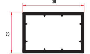
ZİR8661 TEK RAYLI SÜRME KASA YAN KAPATMA PROFİLİ ADAPTER FOR SINGLE RAILED SLIDING FRAME PROFILE ZİR8662 (RENKLİ/COLORED)
