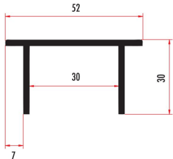
YARUK1 U KAPATMA PROFİLİ U CLOSER PROFILE YARUK2 (RENKLİ/COLORED)
