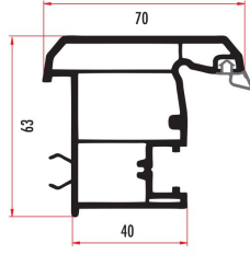
YARP21 PLUS HAREKETLİ ORTA KAYIT PROFİLİ PLUS MOVABLE MULLION PROFILE YARP22 (RENKLİ/COLORED)
