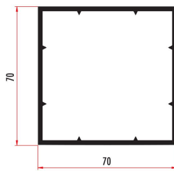
YARK70701 70 X 70 KUTU PROFİLİ 70 X 70 BOX PROFILE YARK70702 (RENKLİ/COLORED)
