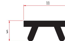
ZİR8651 SÜRME SERİ RAY KAPATMA PROFİLİ RAIL CLOSER ZİR8652 (RENKLİ/COLORED)
