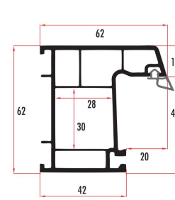
ENR62311 62 MM 3 ODACIKLI KASA / FRAME PROFILE ENR62312 (RENKLİ/COLORED)
