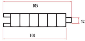
YARP11 PANEL PROFİL PANEL PROFILE YARP12 (RENKLİ/COLORED)
