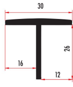
YARTK1 DAR T KAPAMA PROFİLİ T CLOSER PROFILE YARTK2 (RENKLİ/COLORED)
