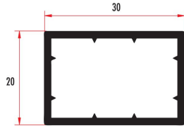
ZİR8661 TEK RAYLI SÜRME KASA YAN KAPATMA PROFİLİ ADOPTER FOR SINGLE RAILED SLIDING FRAME PROFILE ZİR8662 (RENKLİ/COLORED)
