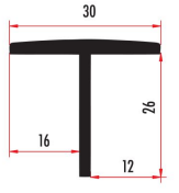
YARTK1 DAR T KAPAMA PROFİLİ T CLOSER PROFILE YARTK2 (RENKLİ/COLORED)
