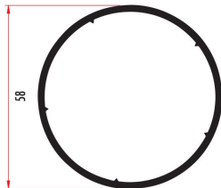
YARA41 BORU PROFİLİ PIPE PROFILE YARA42 (RENKLİ/COLORED)
