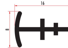
YARI62B1 FIX 1 BİRLEŞİM PROFİLİ CONNECTION PROFILE FOR 62 MM SERİ YARI62B2 (RENKLİ/COLORED)
