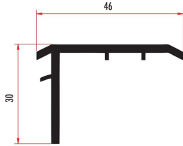
YARI1K1 L ADAPTOR PROFİLİ L ADAPTOR PROFILE YARI1K2 (RENKLİ/COLORED)
