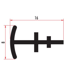
YARI62B1 FIX 1 BİRLEŞİM PROFİLİ CONNECTION PROFILE FOR 62 MM SERİE YARI62B2 (RENKLİ/COLORED)
