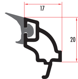
CAM5421 24 MM DEKORATİF ÇİFT CAM ÇİTASI 24 MM DECORATIVE GLAZING BEAD CAM5422 (RENKLİ/COLORED)
