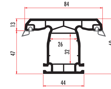
ATL60421 60 MM 4 ODACIKLI SUPER ORTA KAYIT SUPER MULLION PROFILE ATL60422 (RENKLİ/COLORED)
