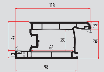
TRU60351 60 MM 3 ODACIKLI KAPI KANAT DOOR SASH PROFILE TRU60352 (RENKLİ/COLORED)
