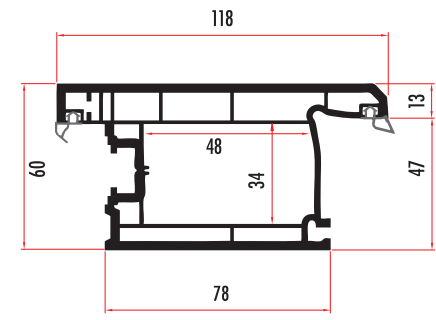
TRU60361 60 MM. 3 ODACIKLI DIŞA AÇILIM PROFİLİ / OUTWARD OPENING DOOR SASH PROFILE TRU60362 (RENKLİ/COLORED)
